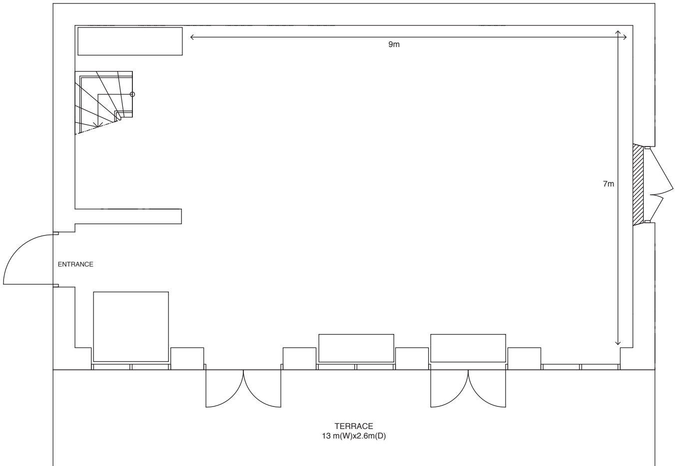
GROUND FLOOR - STILLS & VIDEO STUDIO 80M 2
